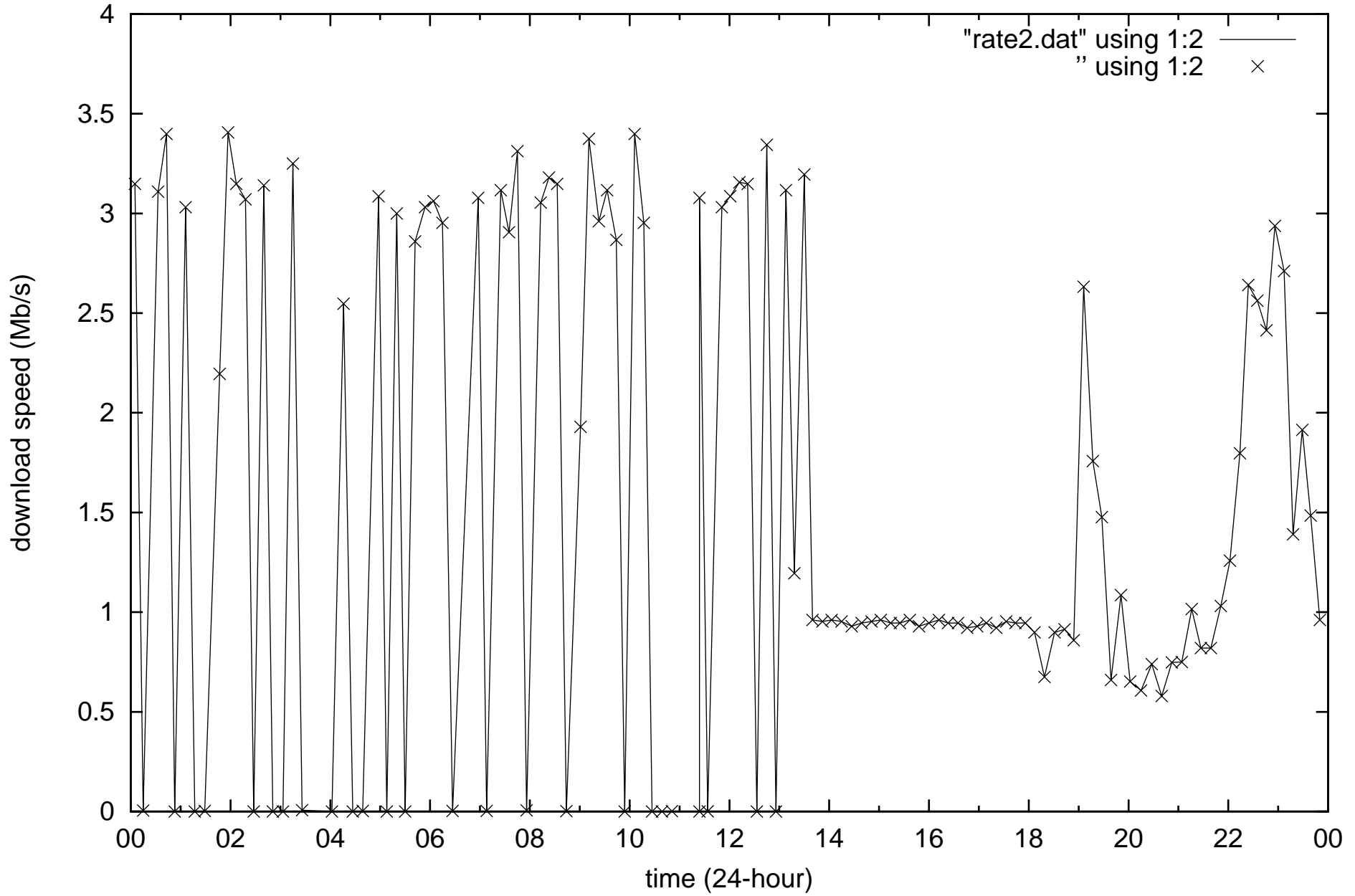
Internet quality Theodore, ACT (TELSTRA ADSL2+) 2017-06-14
