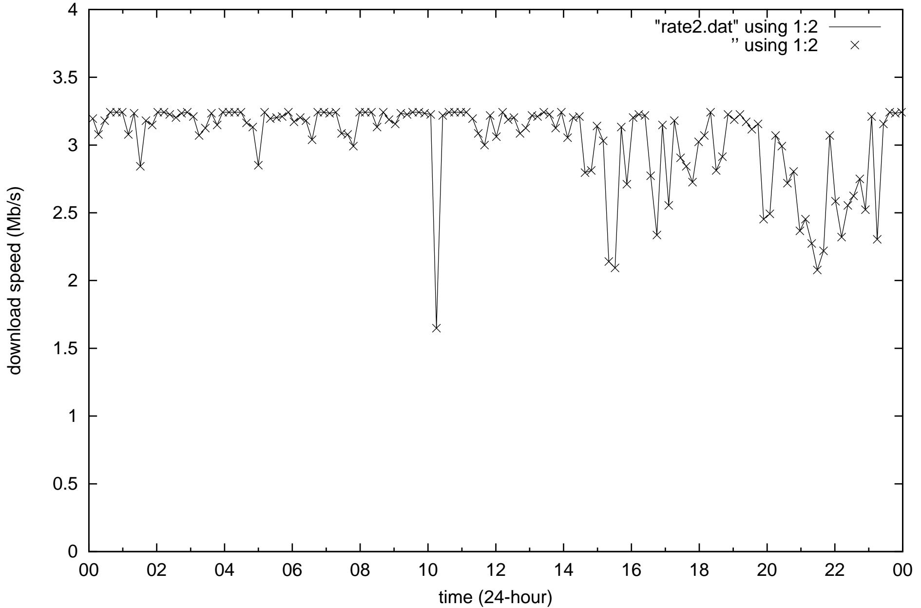
Internet quality Theodore, ACT (TELSTRA ADSL2+) 2017-07-09
