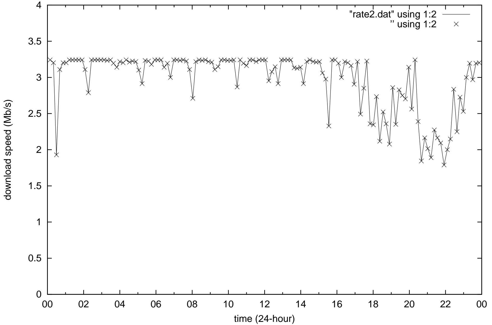
Internet quality Theodore, ACT (TELSTRA ADSL2+) 2017-07-11
