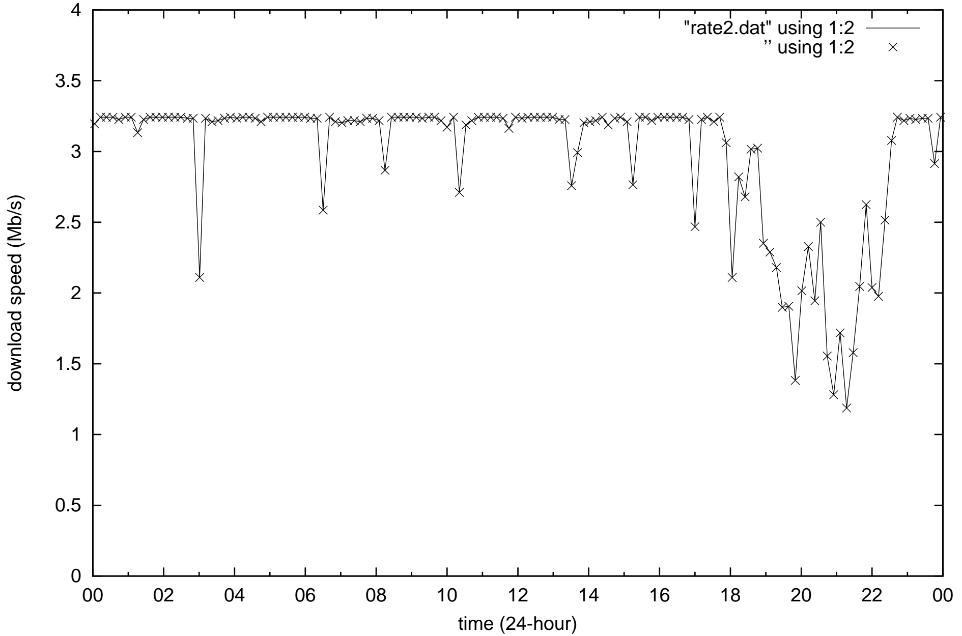
Internet quality Theodore, ACT (TELSTRA ADSL2+) 2017-07-06
