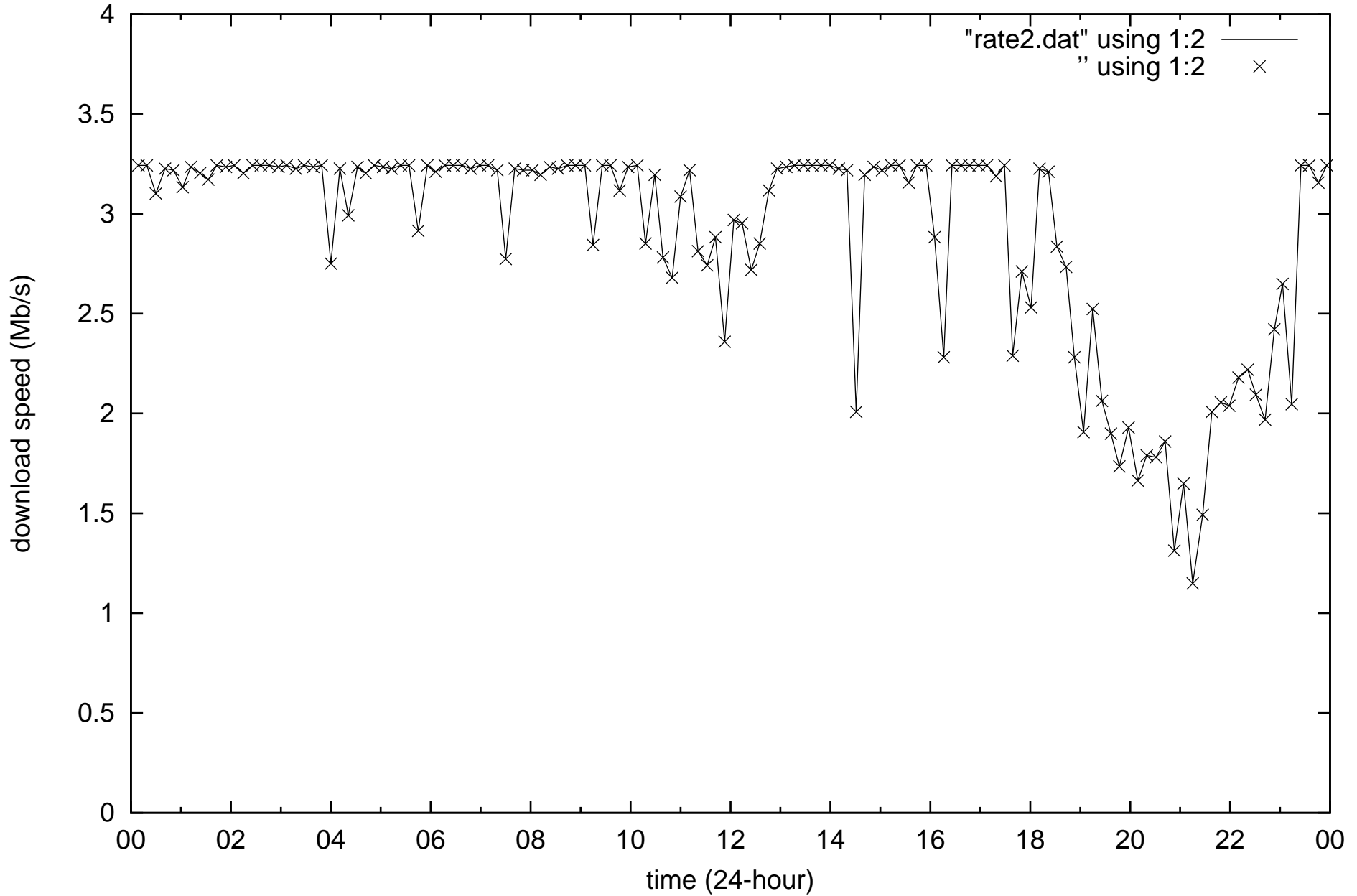
Internet quality Theodore, ACT (TELSTRA ADSL2+) 2017-07-08
