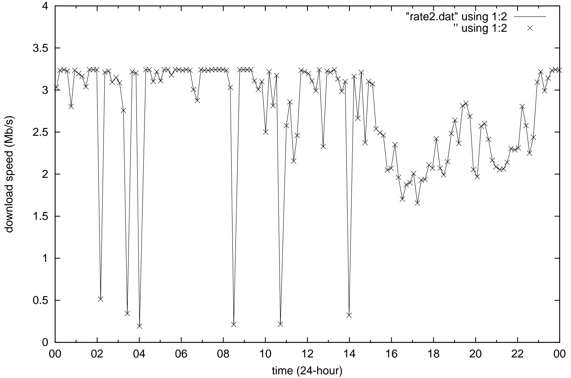
Internet quality Theodore, ACT (TELSTRA ADSL2+) 2017-07-23
