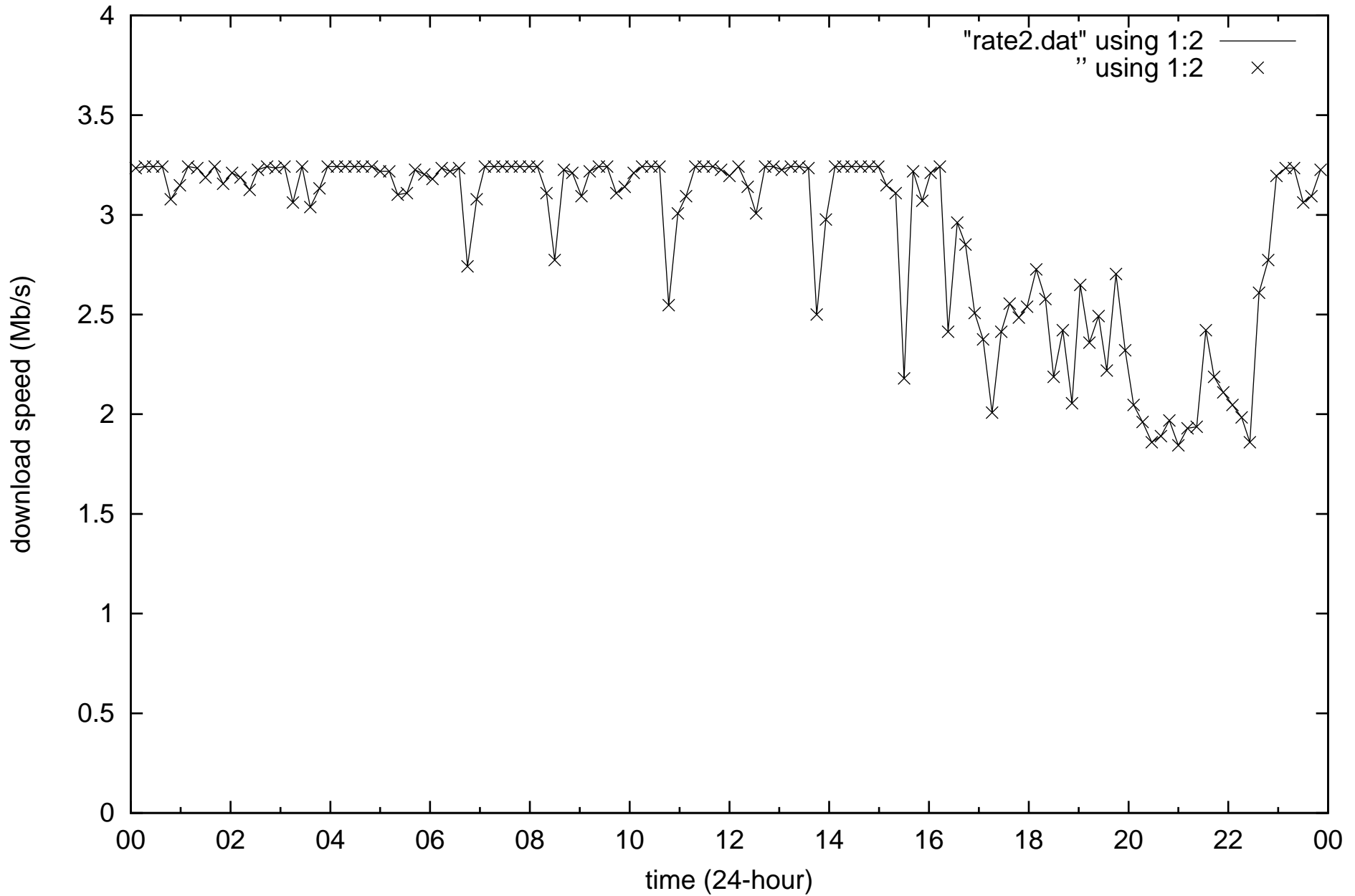
Internet quality Theodore, ACT (TELSTRA ADSL2+) 2017-07-31
