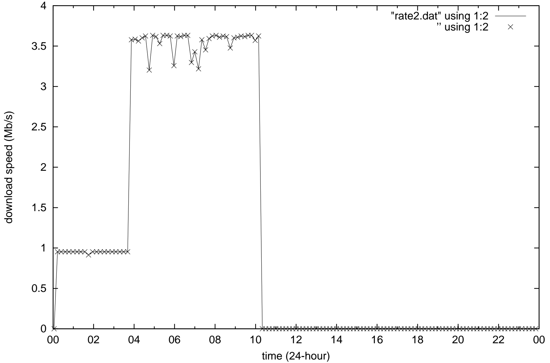
Internet quality Theodore, ACT (TELSTRA ADSL2+) 2017-07-03
