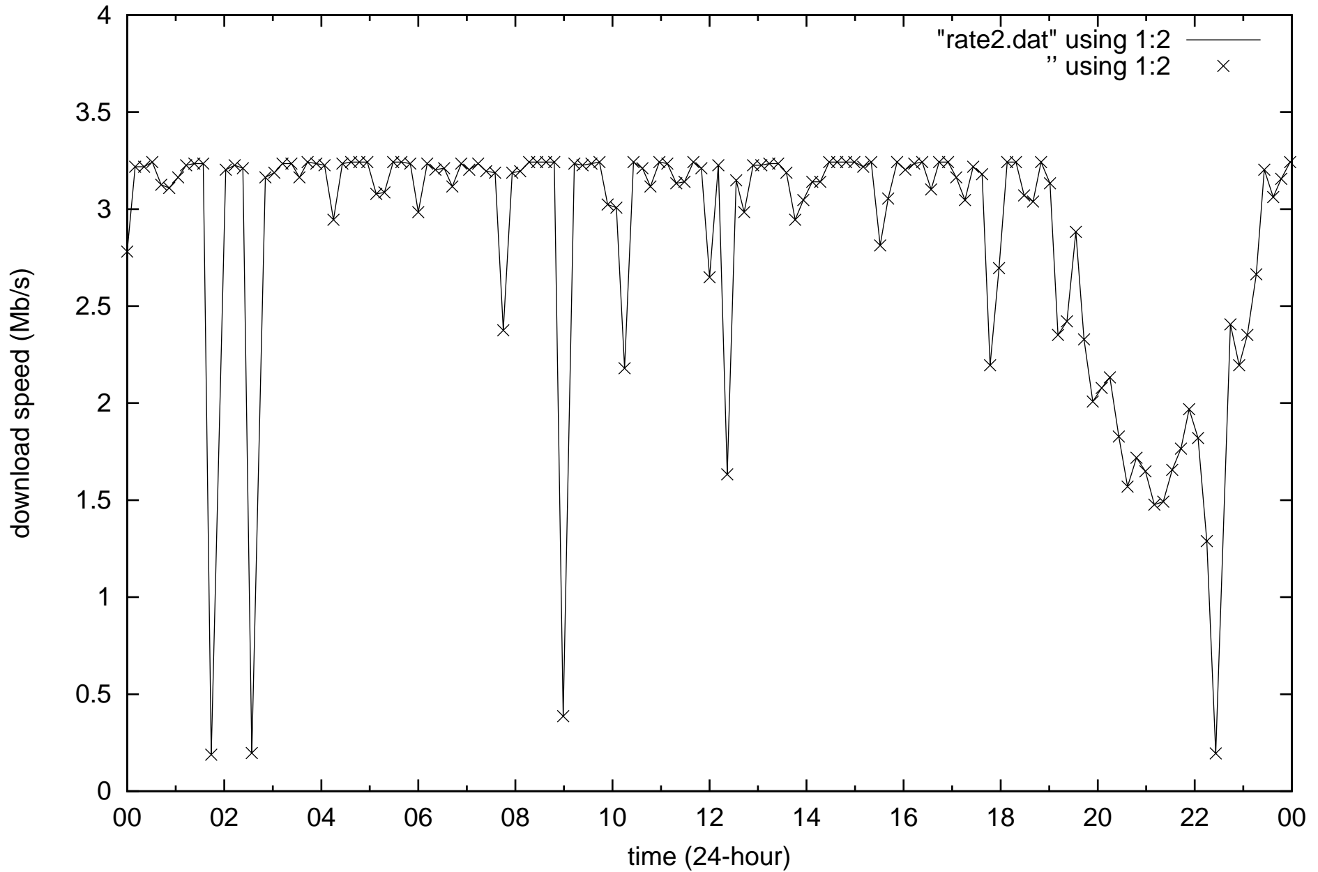
Internet quality Theodore, ACT (TELSTRA ADSL2+) 2017-07-21
