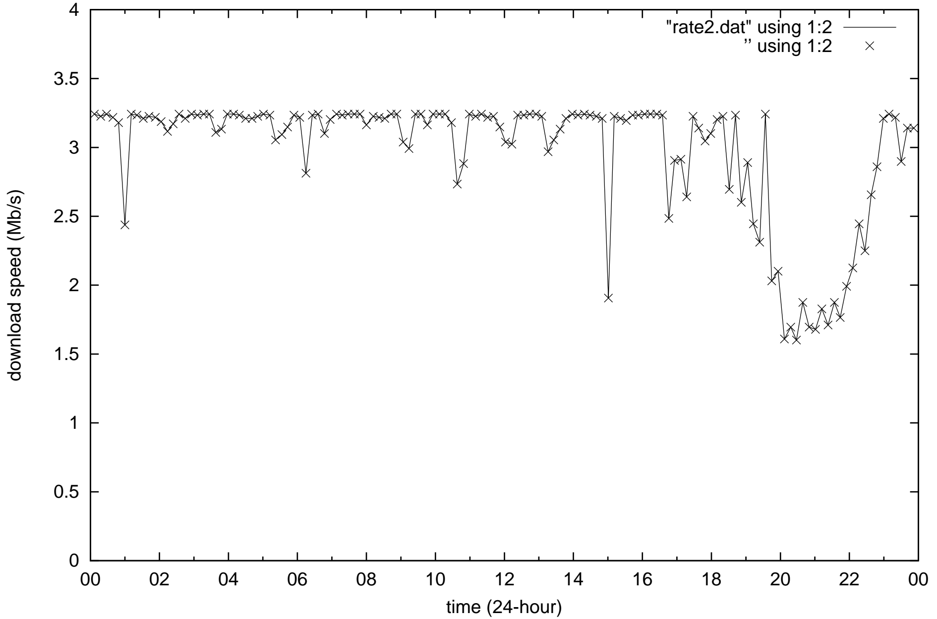
Internet quality Theodore, ACT (TELSTRA ADSL2+) 2017-07-27
