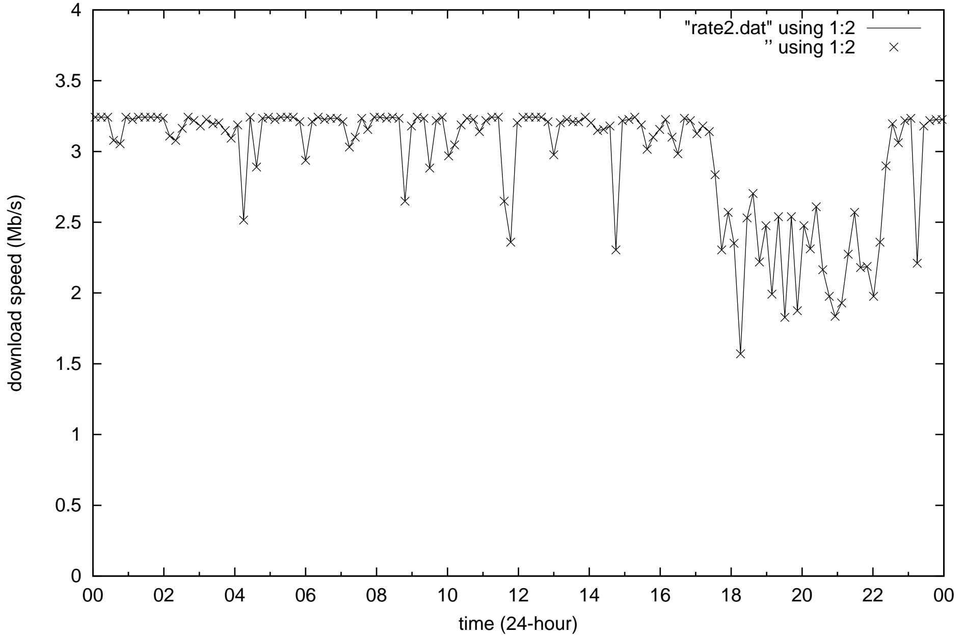
Internet quality Theodore, ACT (TELSTRA ADSL2+) 2017-07-26
