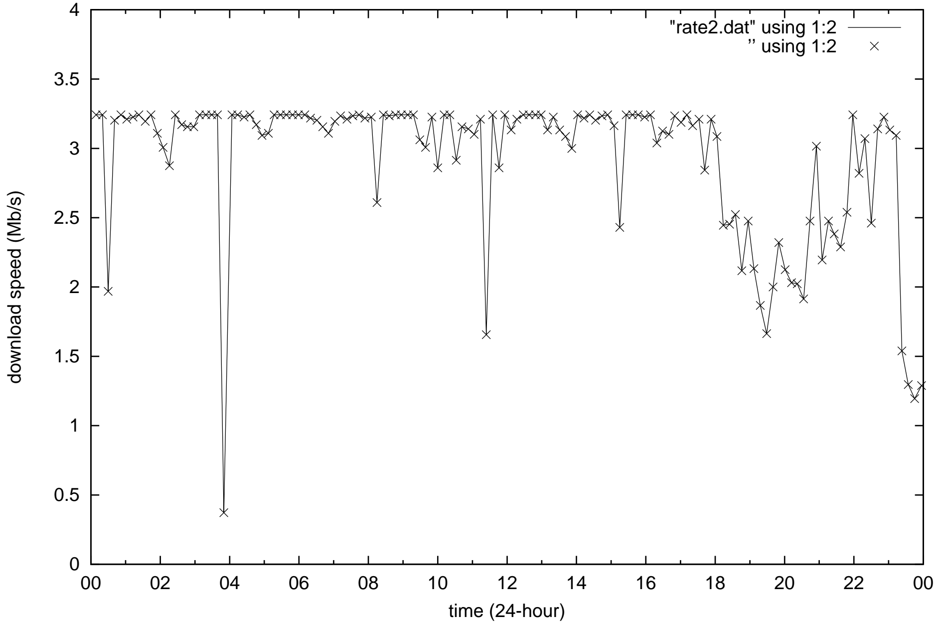
Internet quality Theodore, ACT (TELSTRA ADSL2+) 2017-07-24
