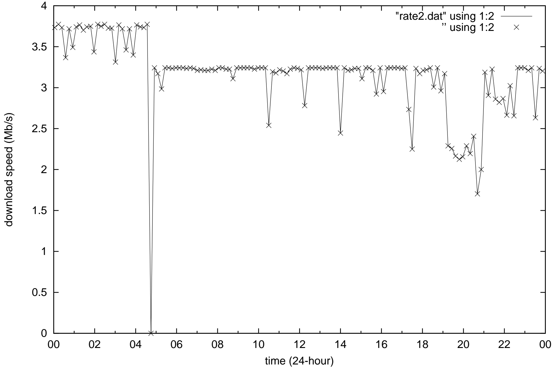
Internet quality Theodore, ACT (TELSTRA ADSL2+) 2017-07-05
