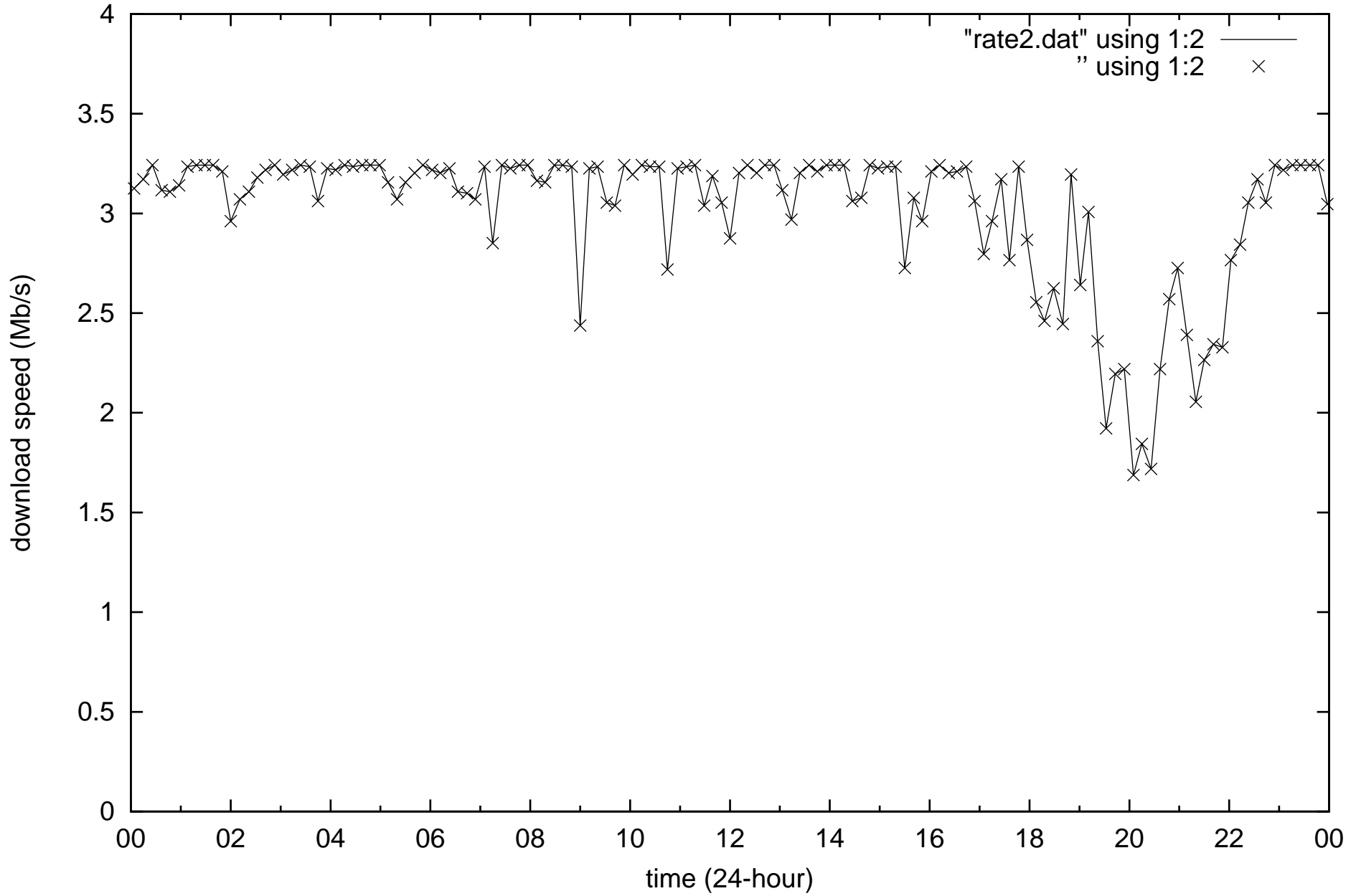
Internet quality Theodore, ACT (TELSTRA ADSL2+) 2017-07-17
