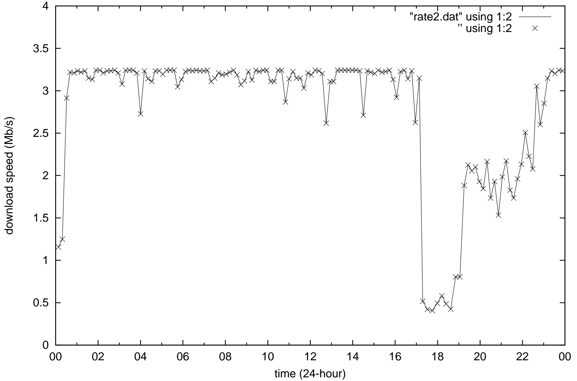
Internet quality Theodore, ACT (TELSTRA ADSL2+) 2017-07-25
