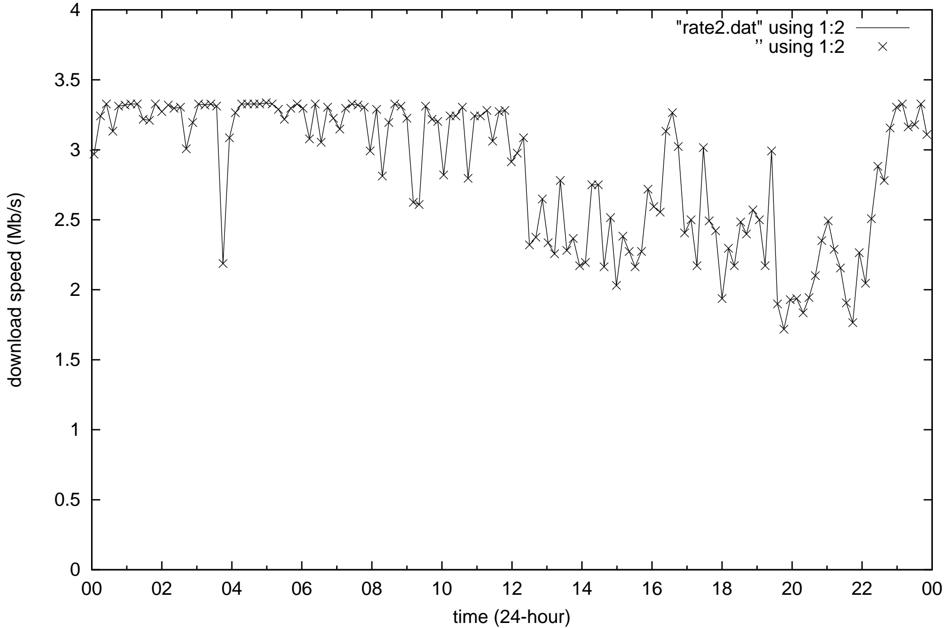
Internet quality Theodore, ACT (TELSTRA ADSL2+) 2017-08-27
