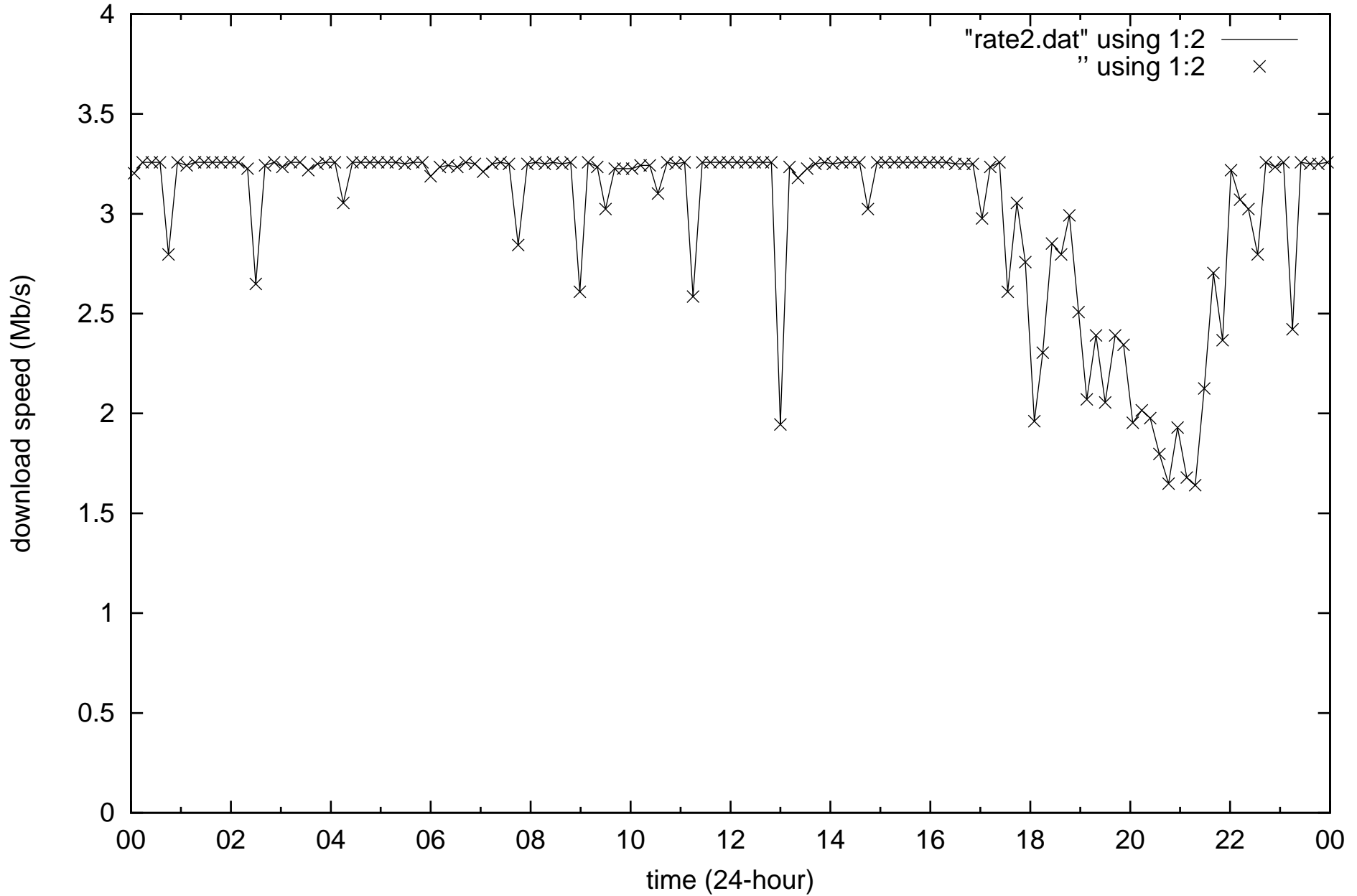
Internet quality Theodore, ACT (TELSTRA ADSL2+) 2017-08-08
