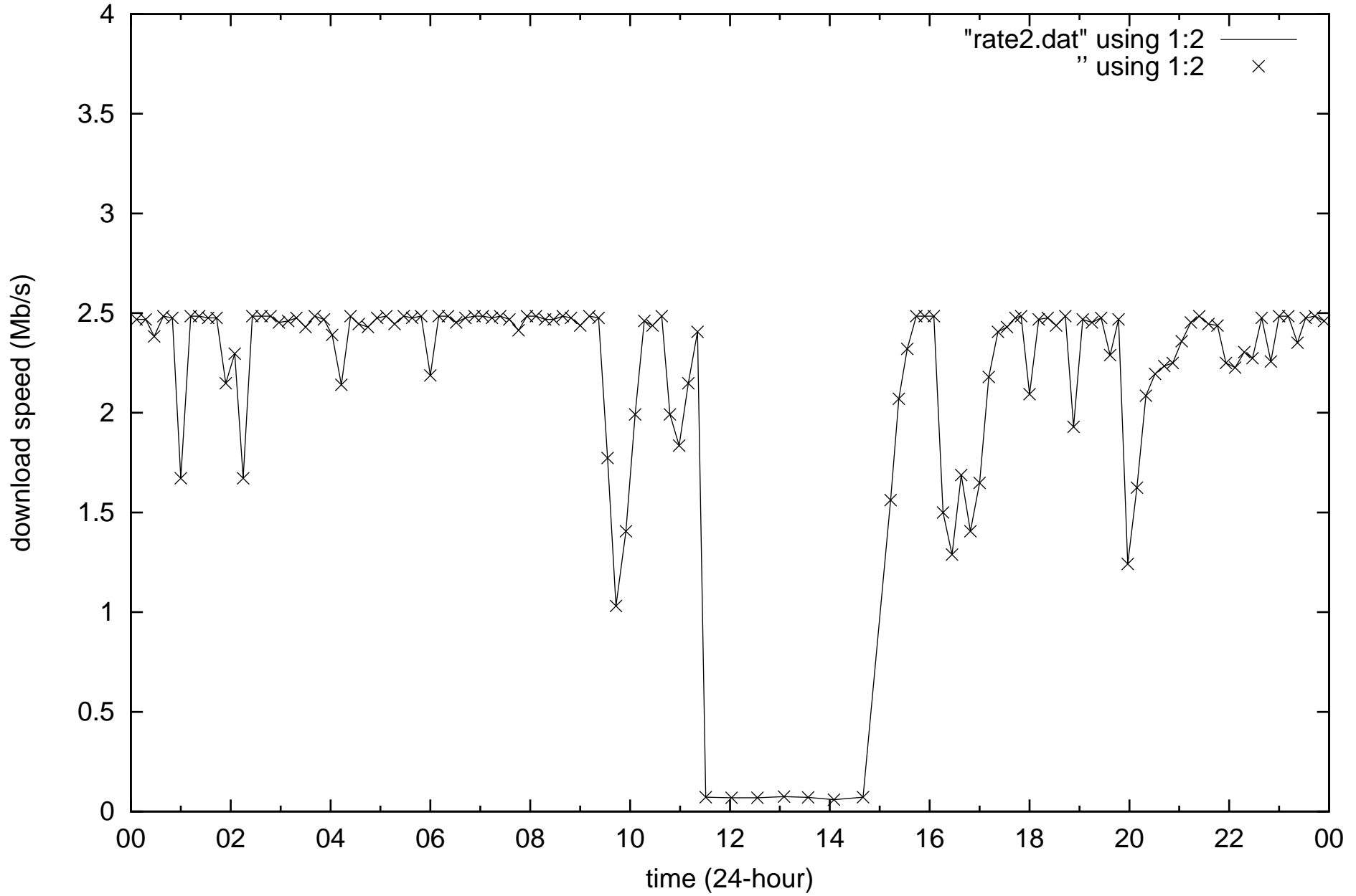
Internet quality Theodore, ACT (TELSTRA ADSL2+) 2017-12-28
