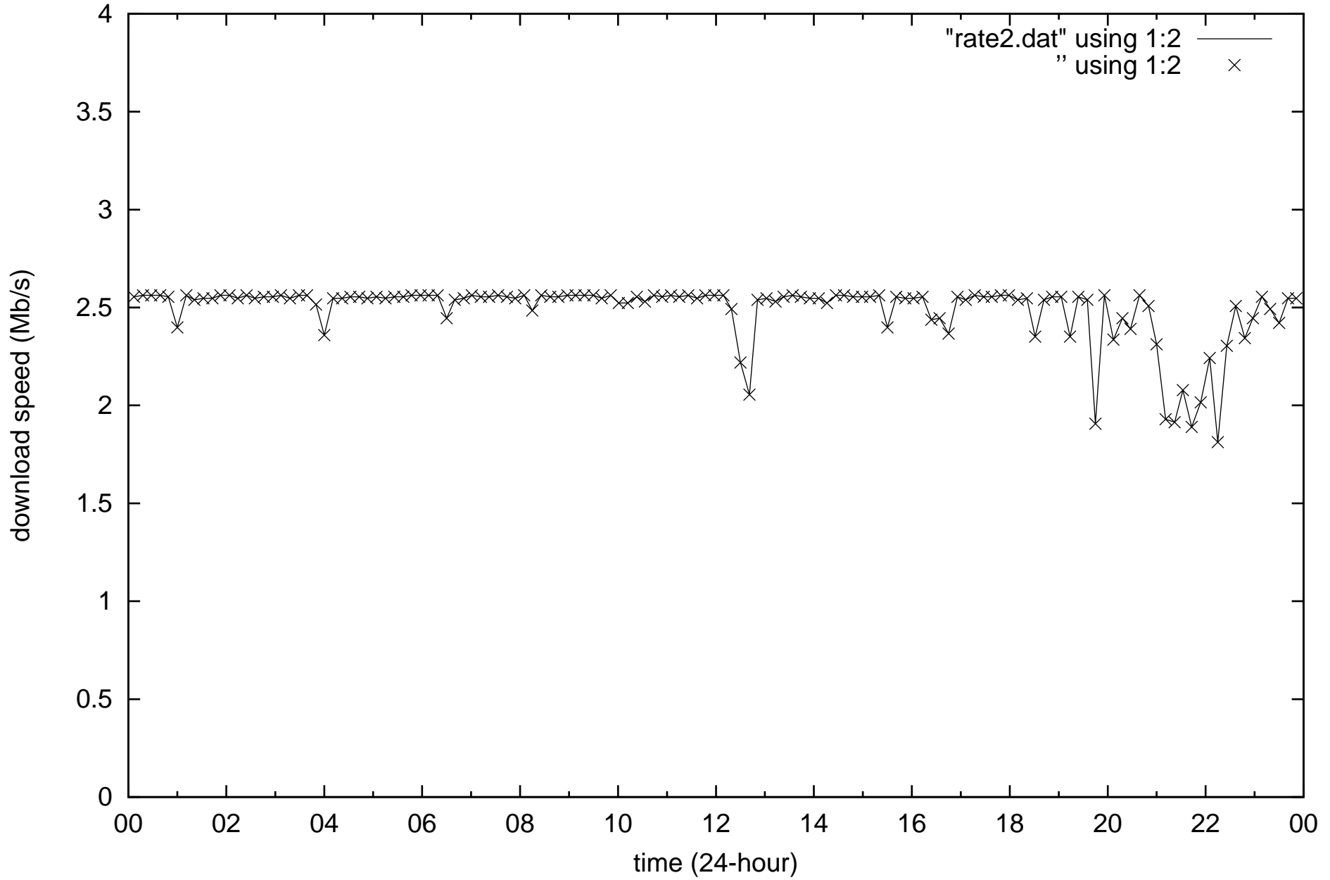
Internet quality Theodore, ACT (TELSTRA ADSL2+) 2017-12-18
