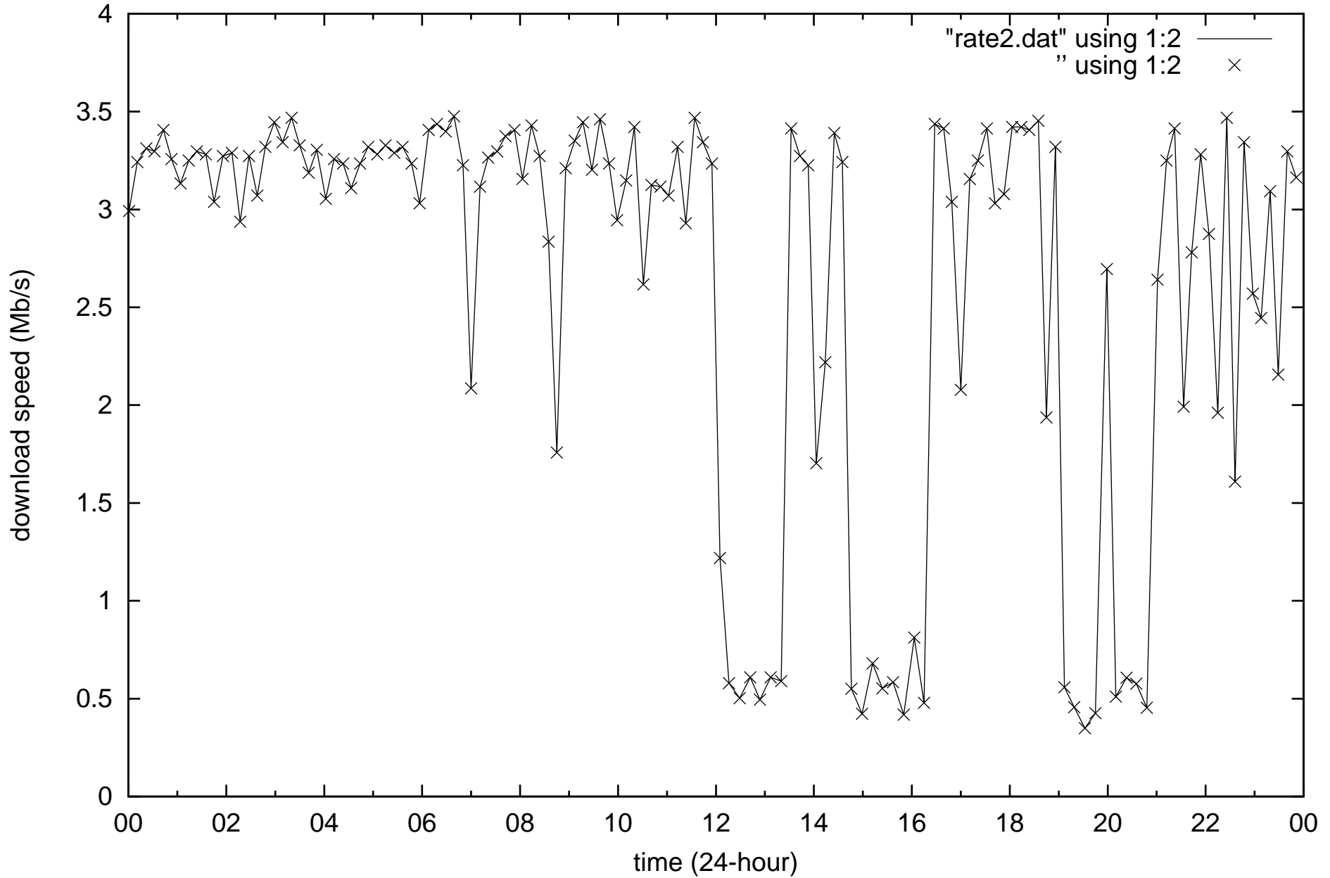
Internet quality Theodore, ACT (TELSTRA ADSL2+) 2018-3-18
