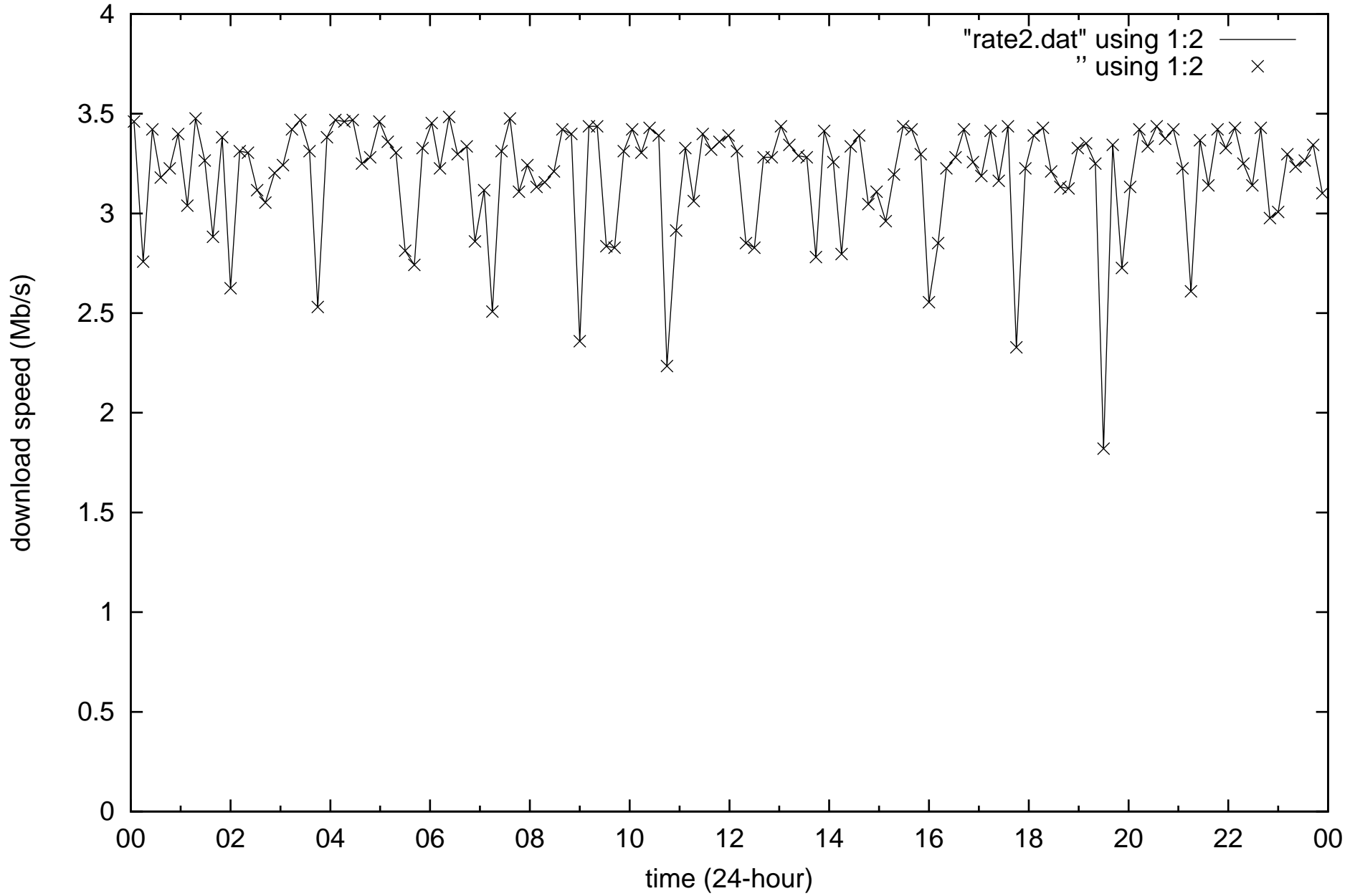
Internet quality Theodore, ACT (TELSTRA ADSL2+) 2018-6-02
