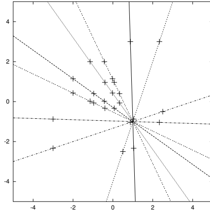
Figure 2: Orbit of (\theta, \phi) = (1/3, 2/5)
