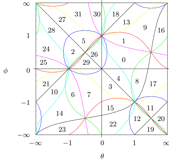
Figure 1: Symmetry boundaries in the \theta\phi -plane
