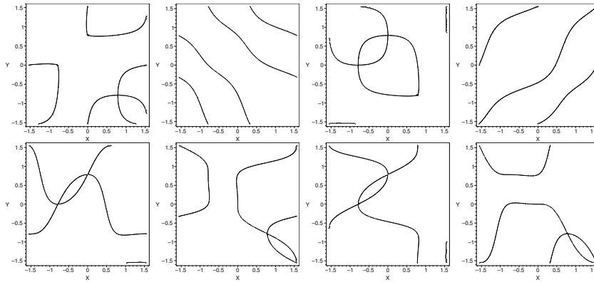
Figure 3: Elliptic curves corresponding to Heron triangles with 2 rational medians ( x = \tan^{-1}(\theta) , y = \tan^{-1}(\phi) )
