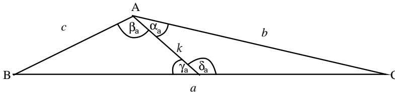
Figure 2: The angles related to Schubert’s parameters
