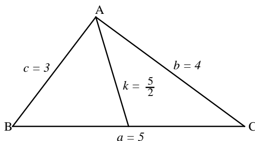
Figure 1: The (5,4,3) right triangle
